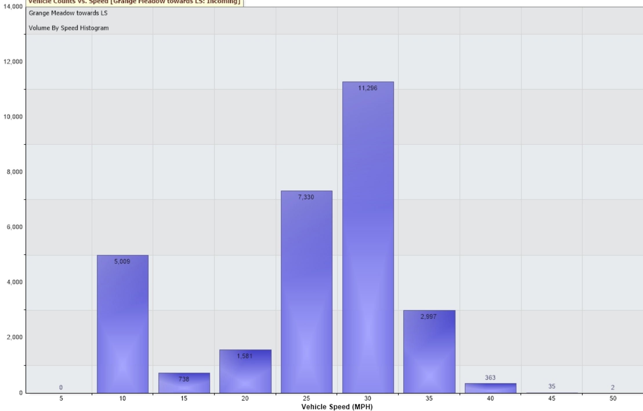
Vehicle Counts Vs. Speed [Grange Meadow towards LS: Incoming]
