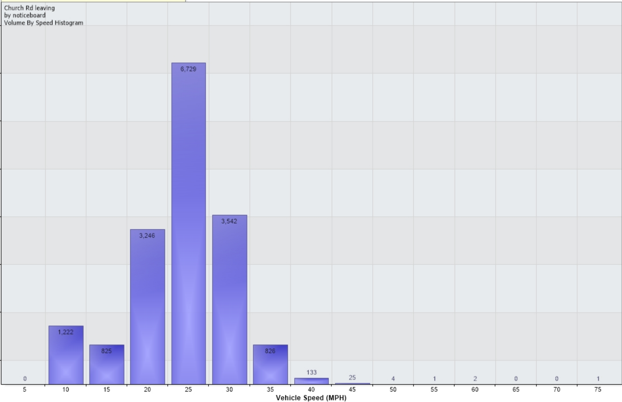
Vehicle Counts Vs. Speed [Church Rd leaving: Incoming]
