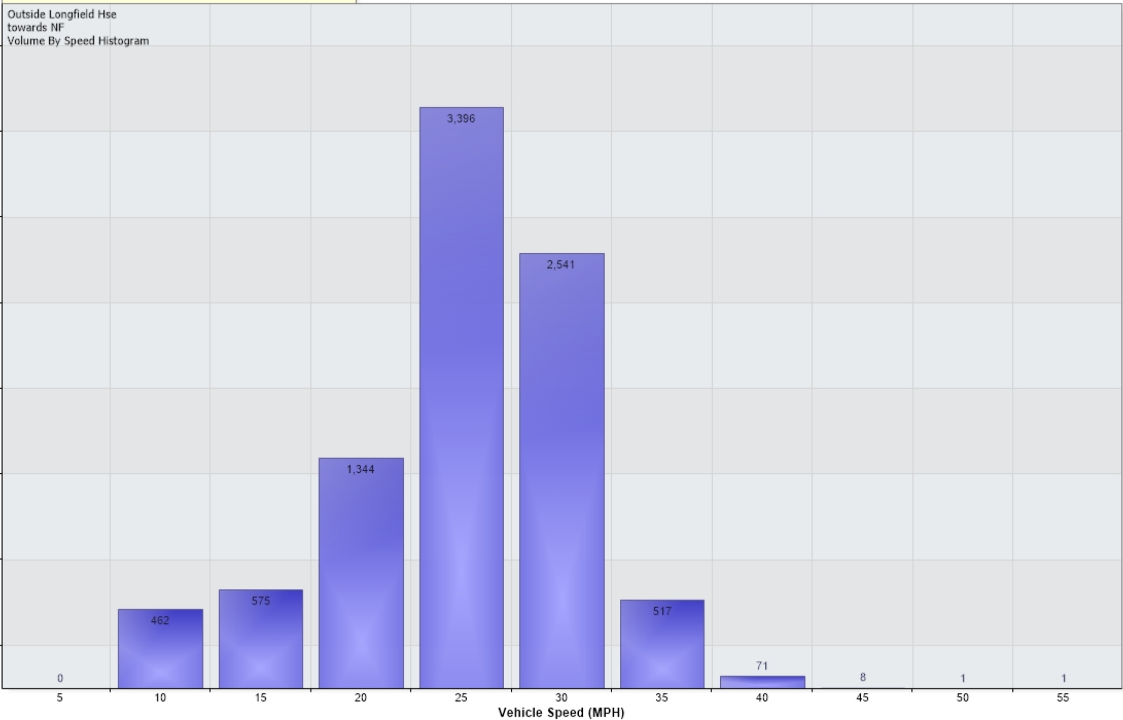
Vehicle Counts Vs. Speed [Outside Longfield Hse : Incoming]
