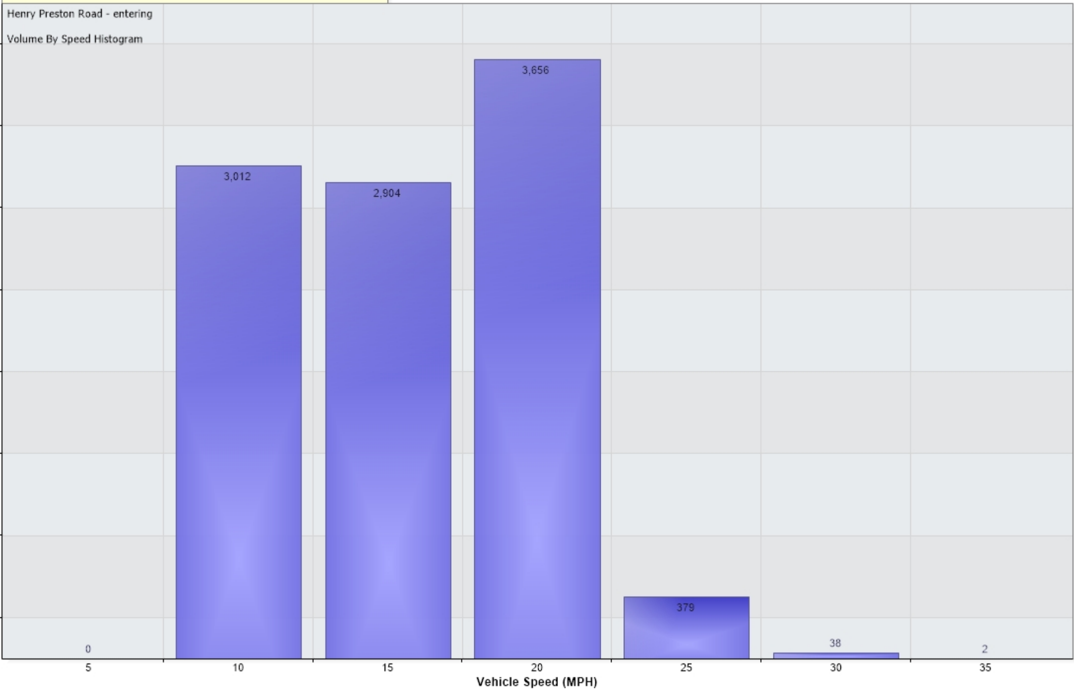
Vehicle Counts Vs. Speed [Henry Preston Road - entering : Incoming]
