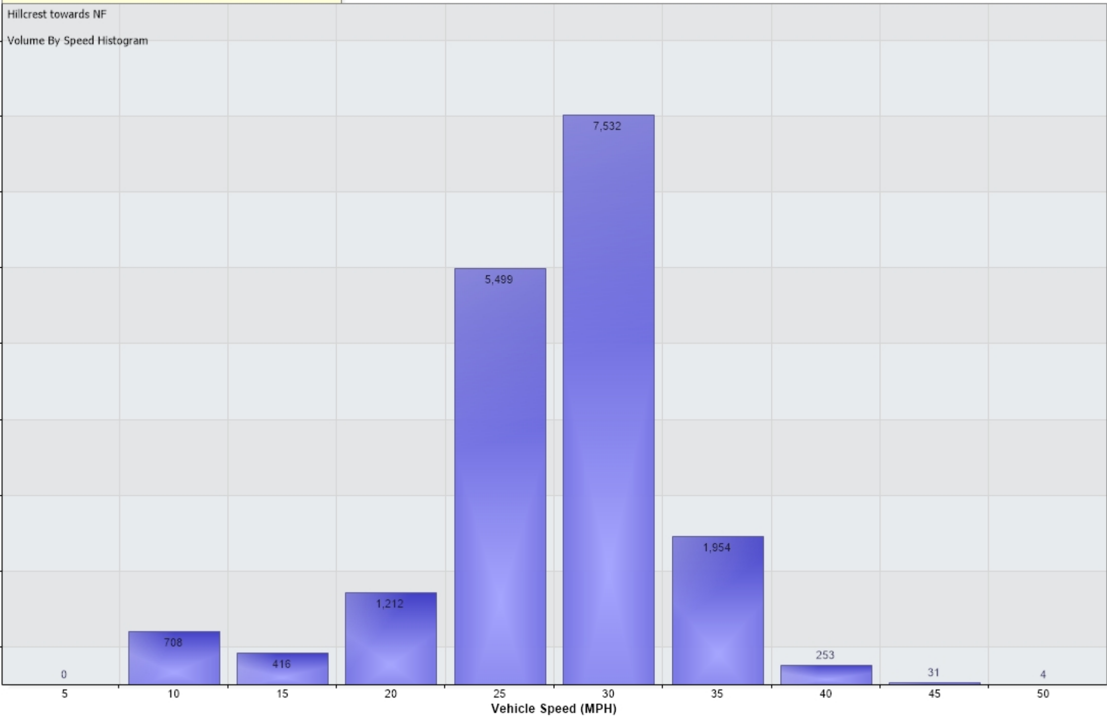
Vehicle Counts Vs. Speed [Hillcrest towards NF: Incoming]
