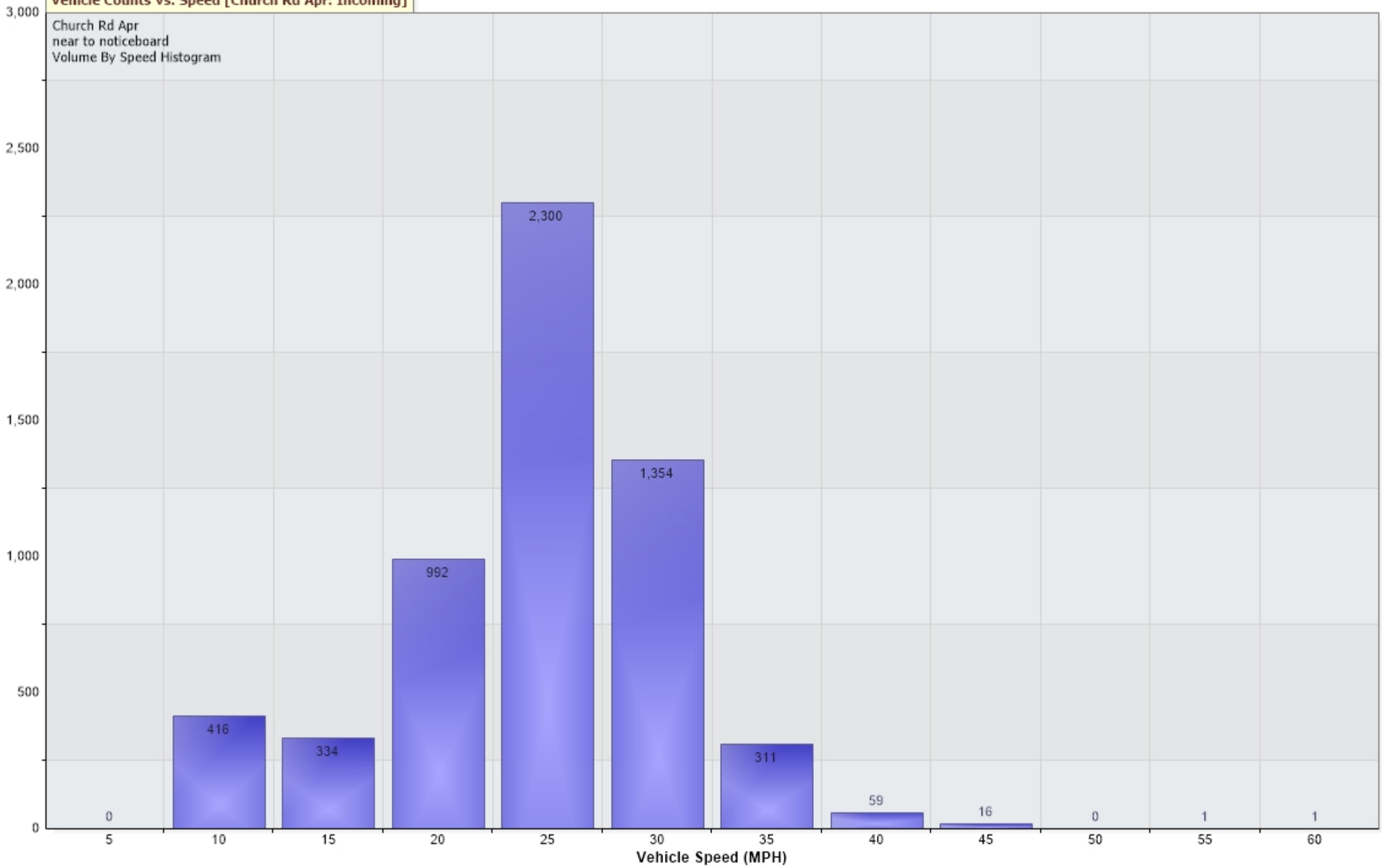
Vehicle Counts Vs. Speed [Church Rd Apr: Incoming]
